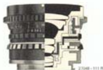
1:4/35 mm PA-CURTAGON®-R
